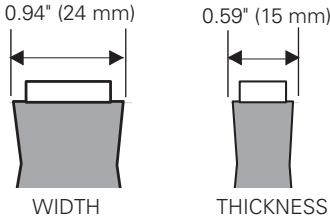
Maximum dimensions of the HDMI connectors
